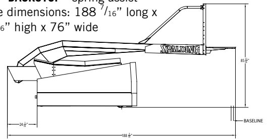
ARENA® BACKSTOP - 10' 8" EXTENSION FOOTPRINT
