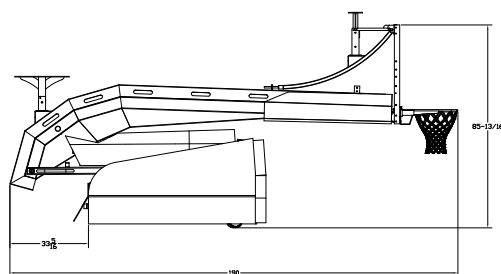
ARENA RENEGADE® BACKSTOP - 10' 8" Extension Footprint
